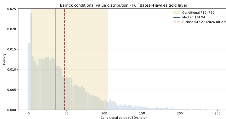
Figure 1: Conditional Barrick value-per-share distribution under the primary Full Bates–Hawkes gold-price scenario. The vertical market reference is the completed B close of USD 47.27 on 27 August 2026. Across 8,192 paths, P10/P50/P90 are USD 3.31/34.94/104.81 and the close lies at the 62.27th percentile. Operations combine Barrick actuals with explicitly labelled Team 4 forecasts; this is not a target-price distribution.
