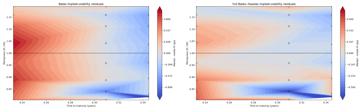
Figure 9.5: Market-minus-model implied-volatility residuals after adding discontinuities: Bates-Poisson (left) and Full Bates-Hawkes (right). The Hawkes layer lowers the current scalar error, while visible clusters remain and residual normality is still rejected.
