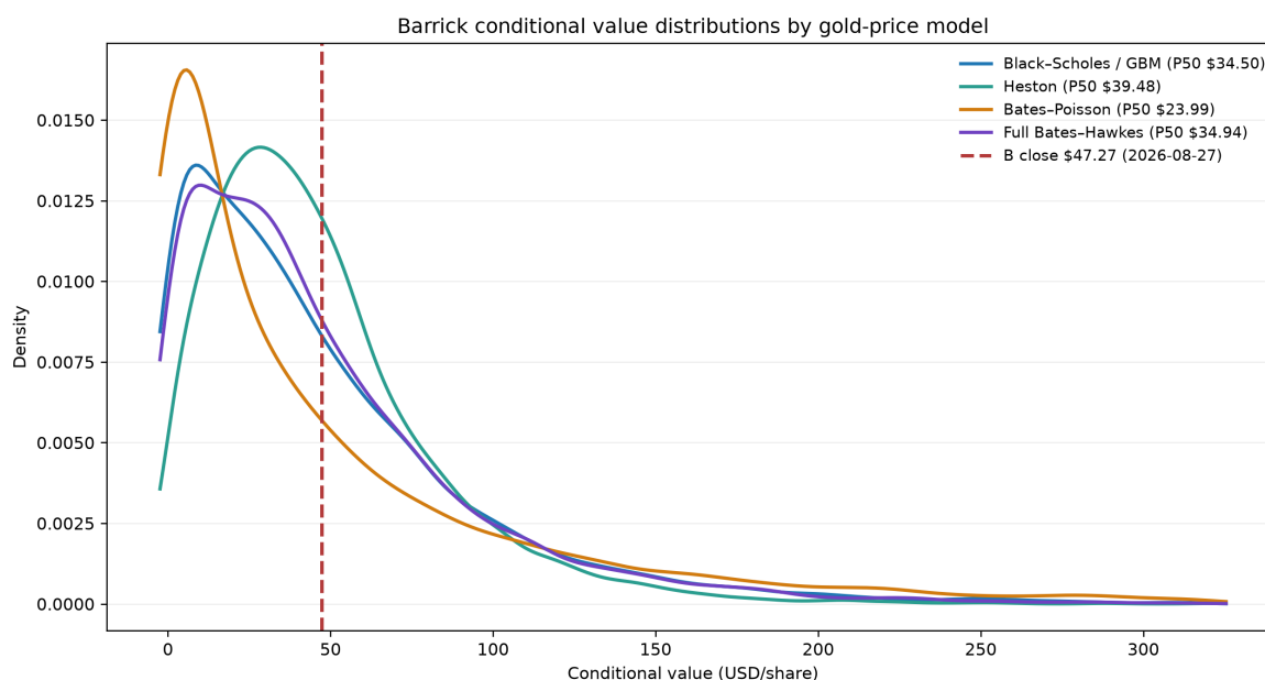
Figure 12.1: Kernel-density comparison of conditional Barrick value per share under the four Chapter 9 gold-price engines. Production, unit cost, DCF, WACC and equity inputs are common; the vertical line is the USD 47.27 completed B close on 27 August 2026.
