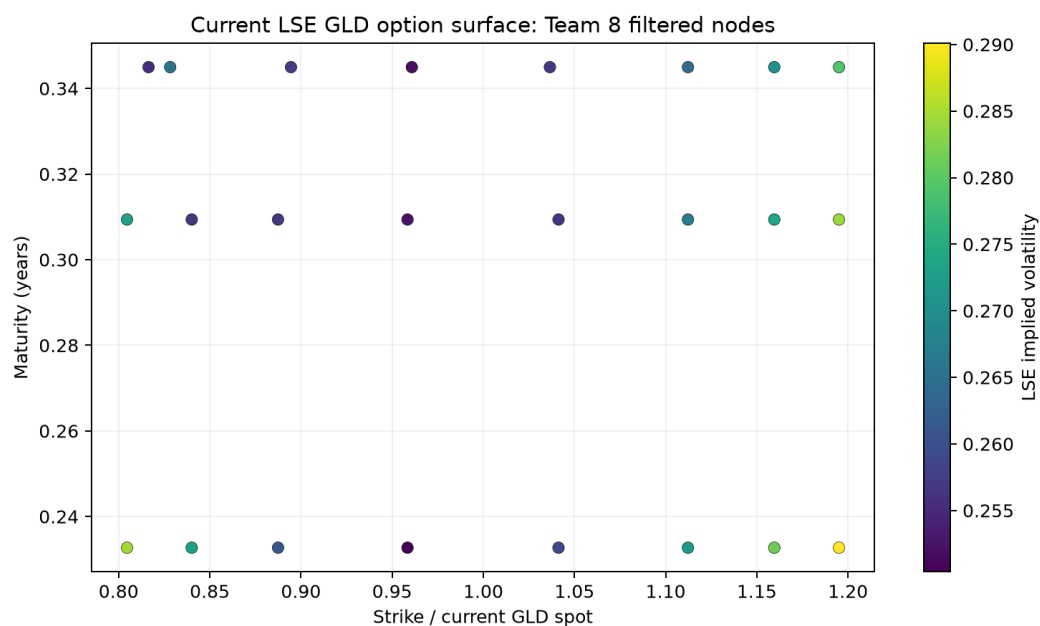
Figure 9.14: Current GLD option nodes retained by the Team 8 filtering and sampling logic. Color denotes LSE implied volatility. The surface is a risk-neutral, IV-mapped object; it is neither a set of contemporaneous traded prices nor a physical forecast of gold in USD/oz.
