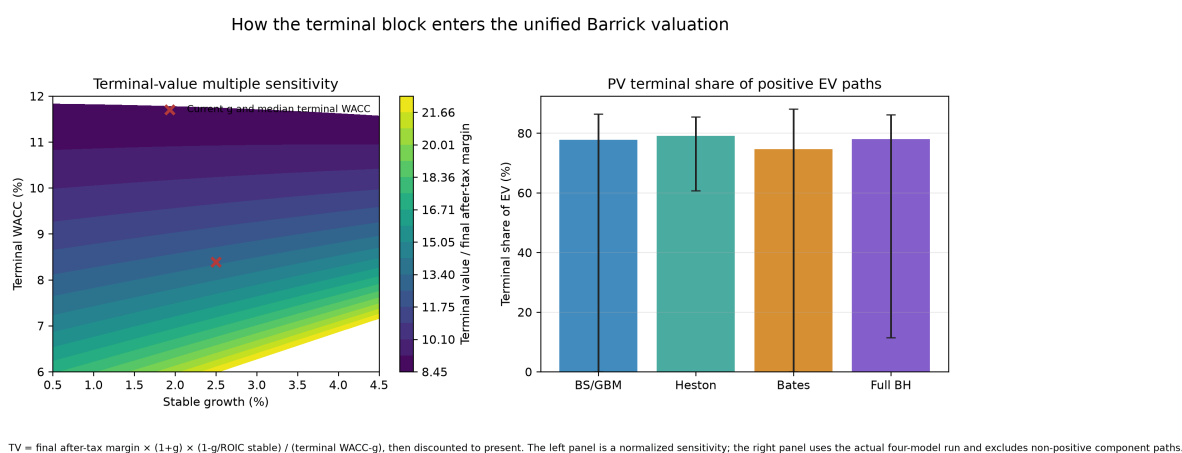
Figure 11.3: Terminal-value mechanics. Left: normalized sensitivity to stable growth and terminal WACC at the current stable ROIC. Right: actual-run P10, median and P90 terminal contribution to positive enterprise-value paths.
