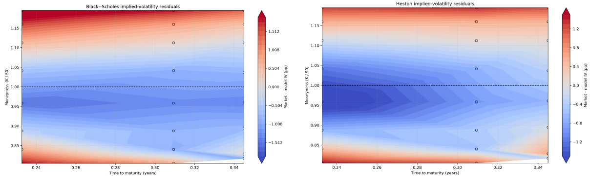
Figure 9.4: Market-minus-model implied-volatility residuals for the two diffusion specifications: Black-Scholes (left) and Feller-constrained Heston (right). Stochastic variance reduces the scalar loss but does not remove structured maturity-moneyness error.
