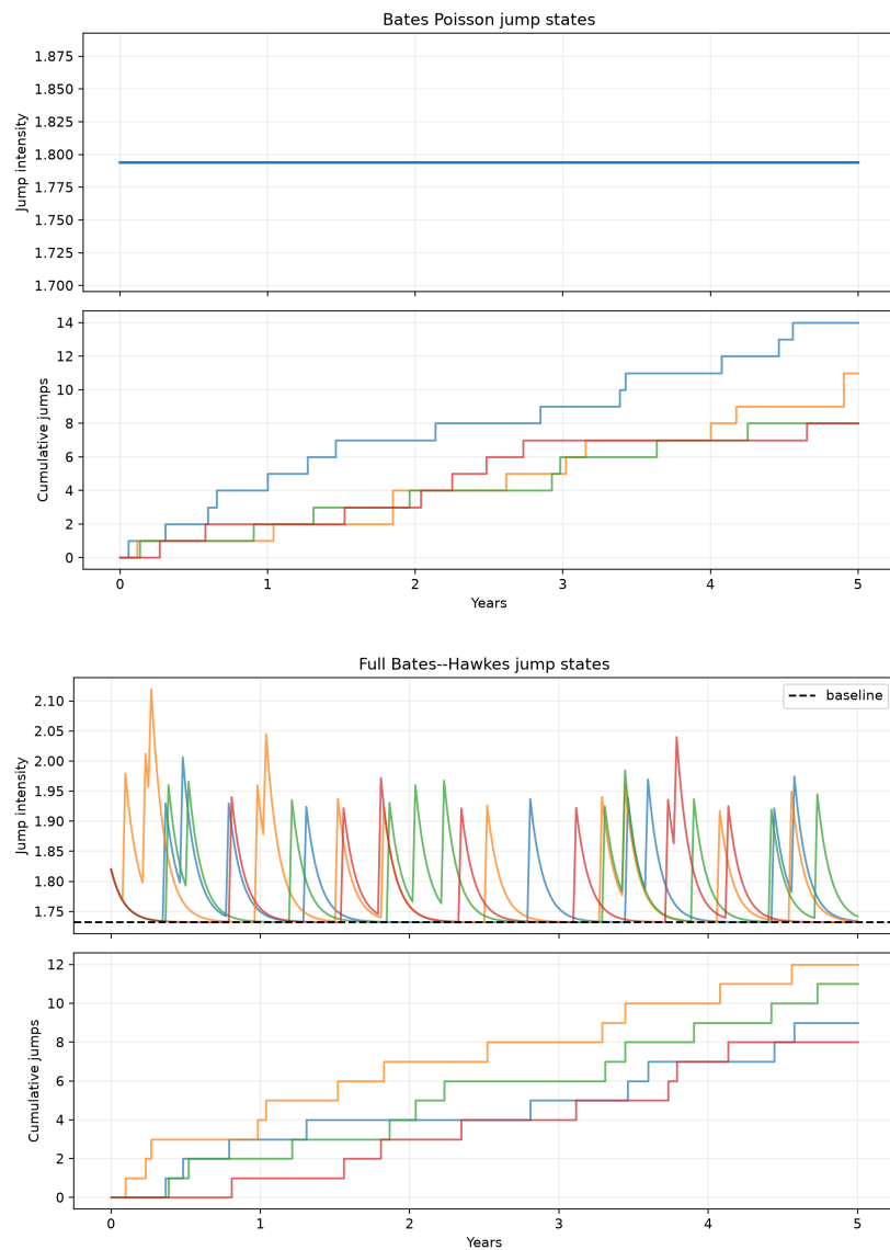
Figure 9.13: Representative jump-state diagnostics. Top: Bates retains a constant Poisson intensity while cumulative counts evolve independently. Bottom: Full Bates-Hawkes intensity rises after arrivals and decays toward its baseline, generating clustered event counts. These path displays explain the state difference behind the tail comparison; they are not additional forecast observations.
