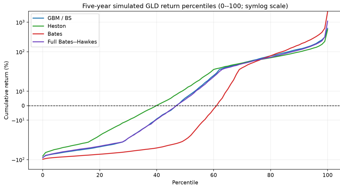
Figure 9.11: All integer percentiles 0–100 of five-year simple GLD returns in the current Team 8 simulation. The symmetric-log scale retains the central distribution while exposing extreme endpoints; the full integer percentile tables remain in the source article rather than being repeated in the thesis.
