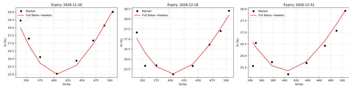
Figure 9.6: Observed and Full Bates-Hawkes implied-volatility smiles across the three sampled expiries. The panel view prevents a low aggregate RMSE from concealing expiry-specific misses, especially at boundary strikes.
