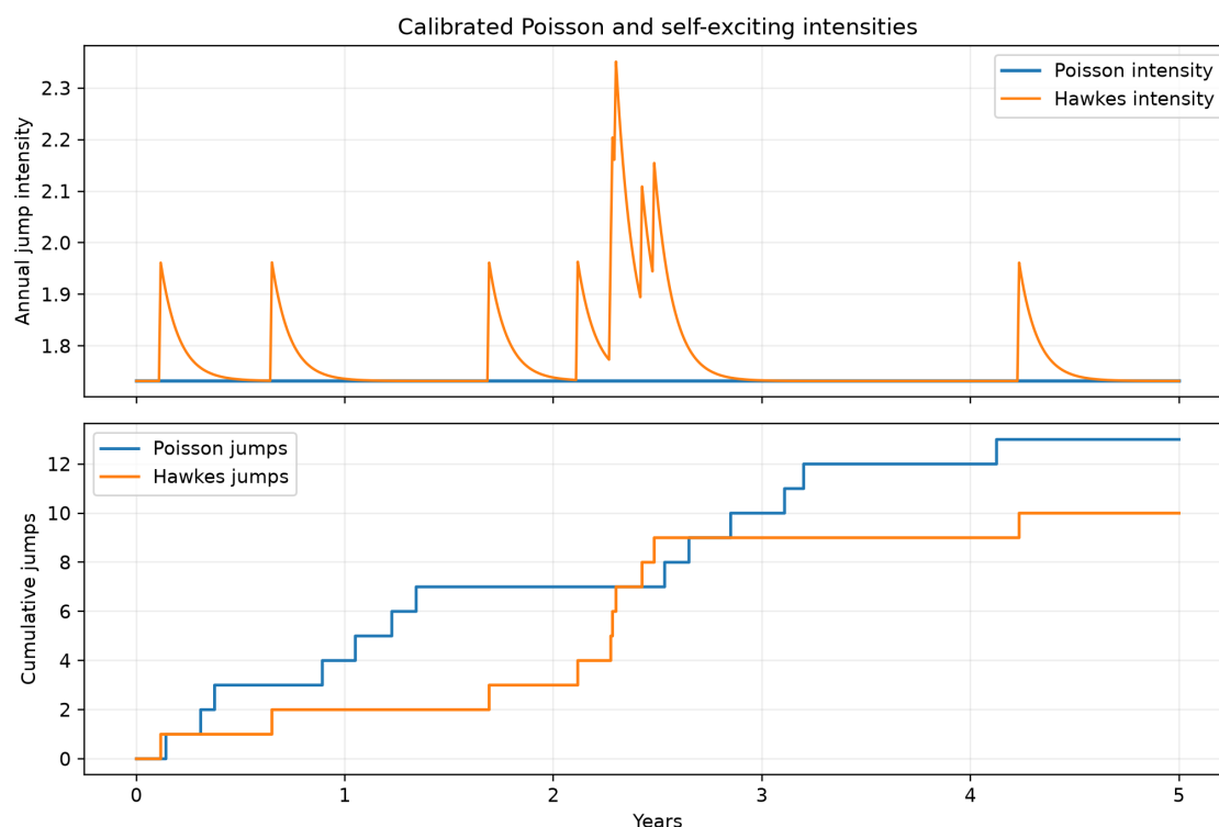
Figure 9.7: Constant-intensity Bates jumps versus self-exciting Bates–Hawkes jumps regenerated from the current calibration. A Hawkes arrival raises near-term intensity, which subsequently decays toward its baseline; the lower panel shows the associated clustered event counts.
