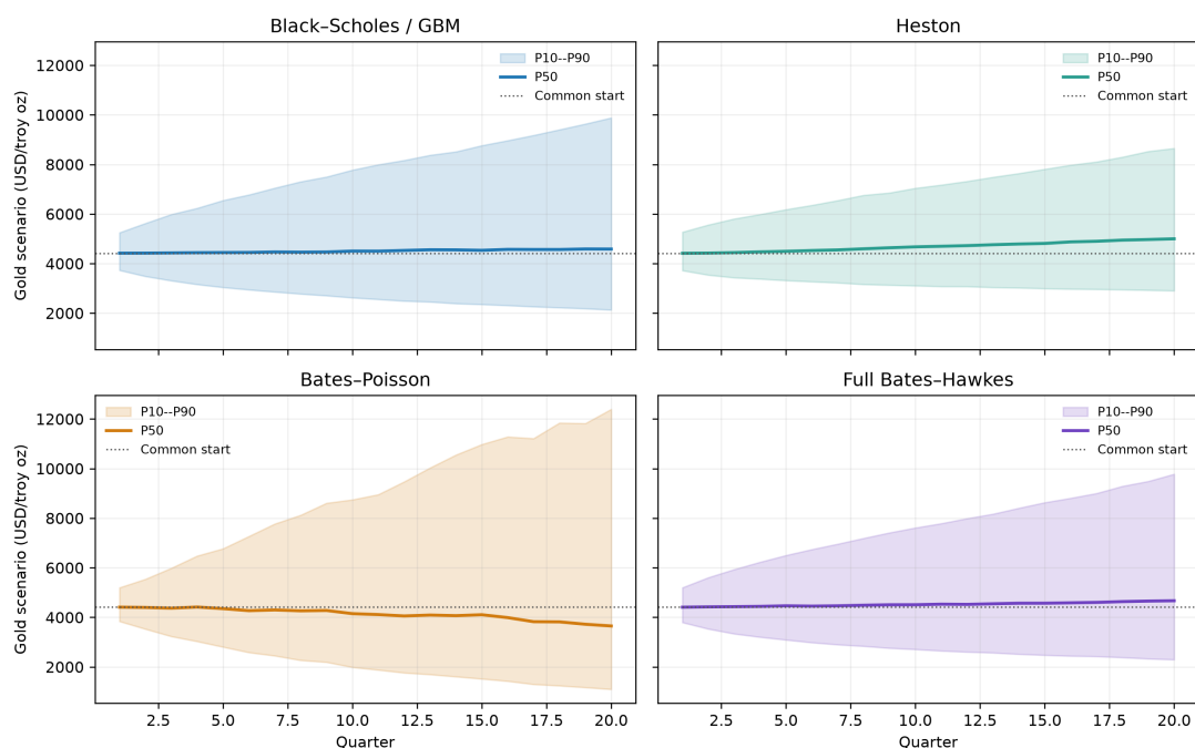
Conditional gold path bands - four option-implied engines
