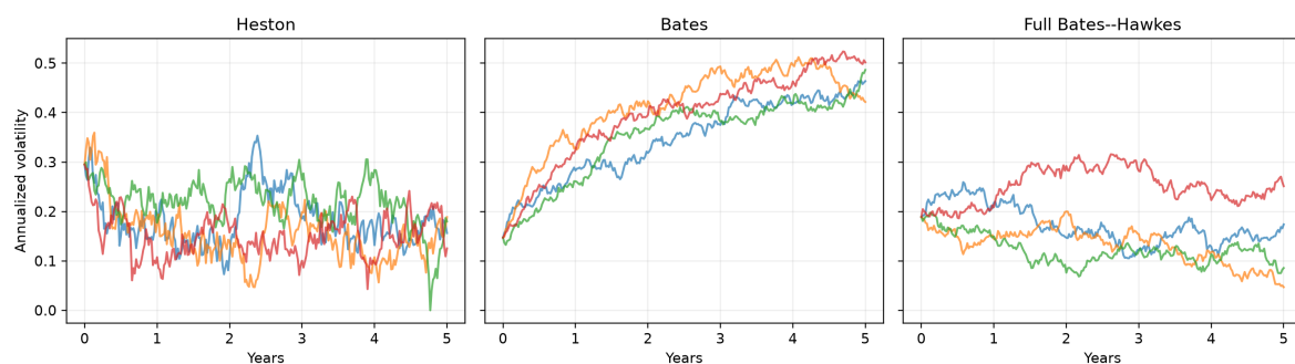
Figure 9.12: Representative annualized stochastic-volatility paths under Heston, Bates and Full Bates–Hawkes on a common scale. The plot verifies that all three richer engines carry a simulated variance state; the jump mechanism does not replace stochastic variance.
